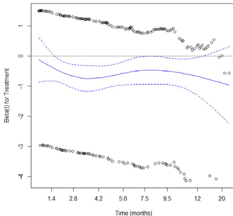
Figure 13. Schoenfeld residuals as a function of time in HER2CLIMB, progression free survival
